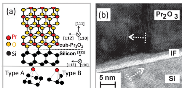
Fig. 5 (a) Atomic model of the cub- \text{Pr}_2\text{O}_3(111)/\text{Si}(111) interface. (b) Cross-sectional HRTEM image of the cub- \text{Pr}_2\text{O}_3(0001)/\text{Si}(111) heterostructure.
